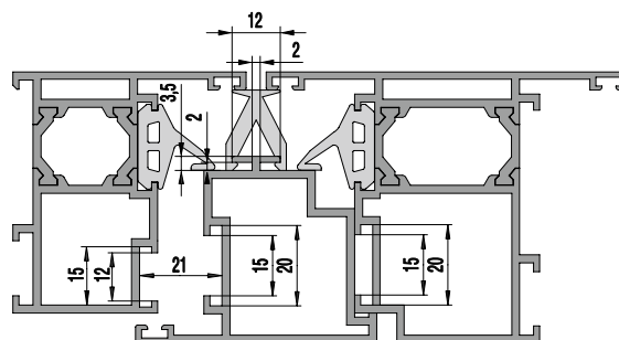
框槽 12/15
