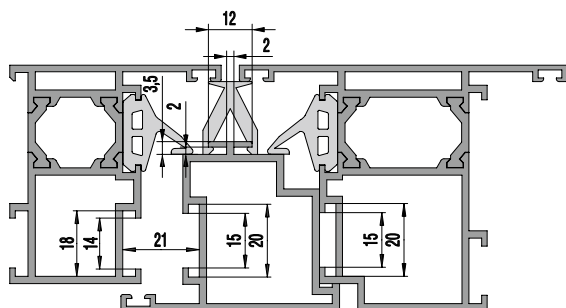
框槽 14/18
