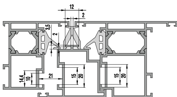
框槽 10/14
