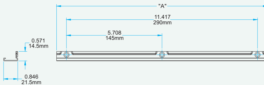
Dual Arm Operator Track 3 Holes
