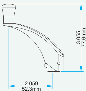
Folding Down Crank 132062
