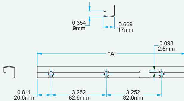
Single Arm Operator Track 3 Holes
