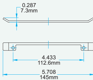
Stud Bracket 19048 (Non-Handed)
