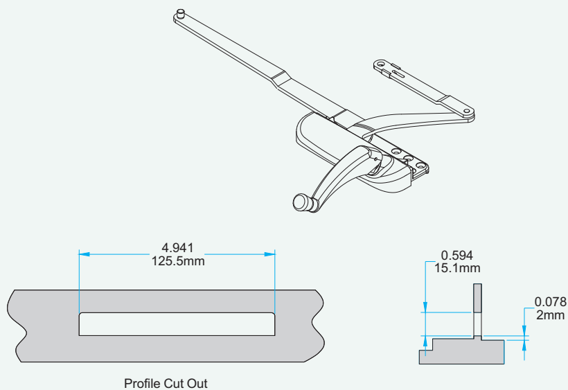
Stud Bracket (Right-Hand Shown)
