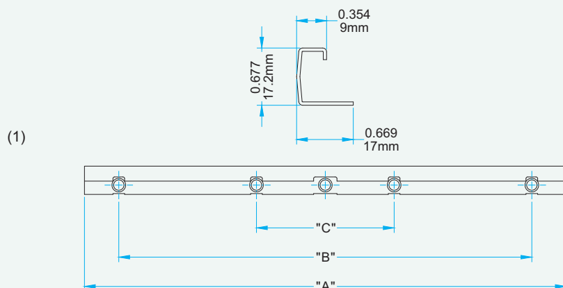
Single Arm Operator Track
