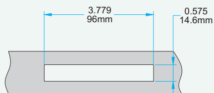
Profile Cut Out (Wood Profile)
