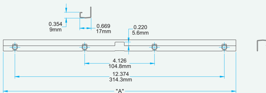
Single Arm Operator Track 4 Holes
