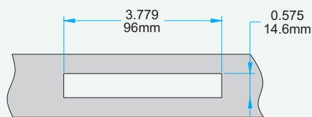
Profile Cut Out (Wood Profile)
