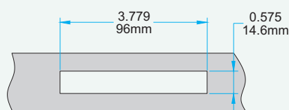
Profile Cut Out (Wood Profile)
