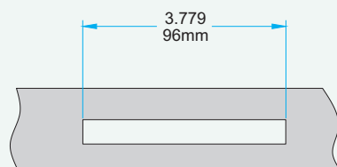
Profile Cut Out (PVC Profile)
