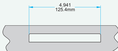
Profile Cut Out
