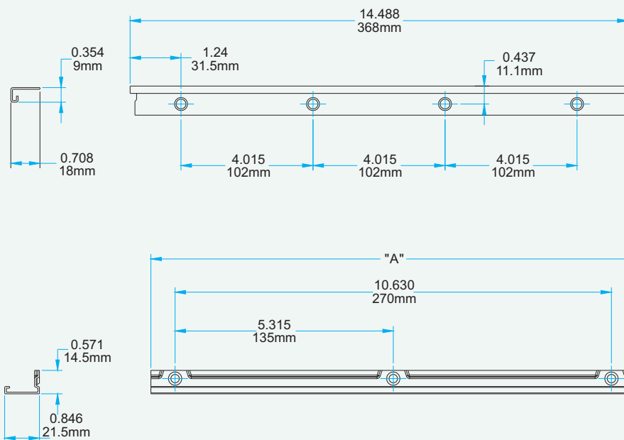
Dual Arm Operator (Low Profile) Track 190056
