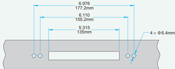
Profile Cut Out
