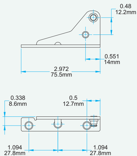
Stud Bracket (Right-Hand Shown)
