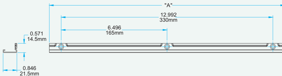
Dual Arm Operator Track 3 Holes
