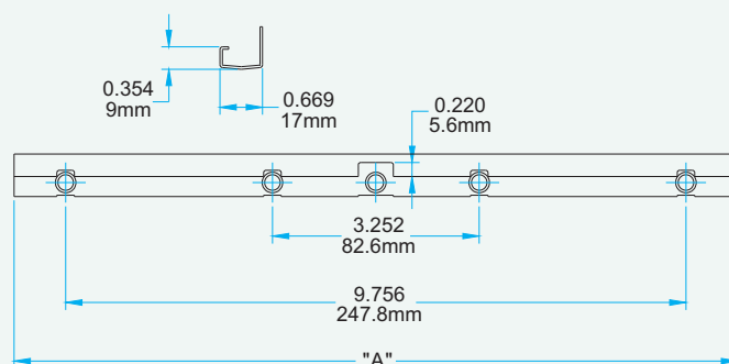
Single Arm Operator Track 5 Holes
