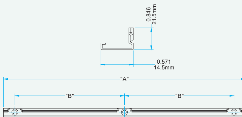
Dual Arm Operator Track 3 Holes
