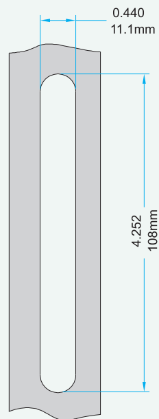
Frame Cut Out
