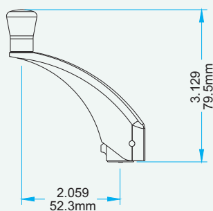
Folding Down Crank 132063
