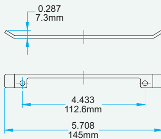
Stud Bracket (Right-Hand Shown)
