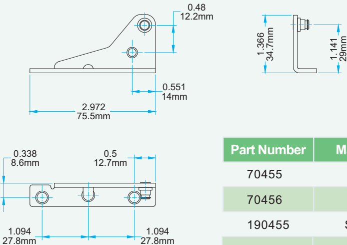
Stud Bracket (Right-Hand Shown)
