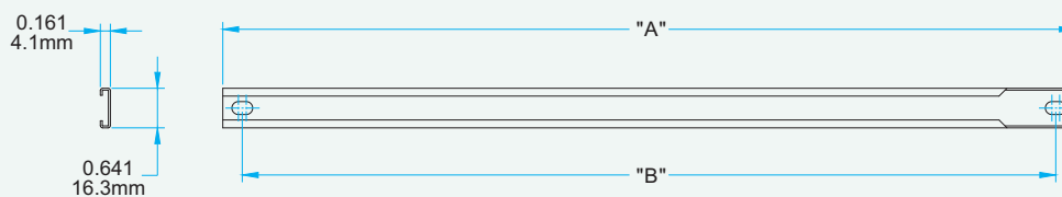
Single Arm Operator Track
