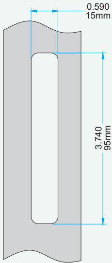
Frame Cut Out
