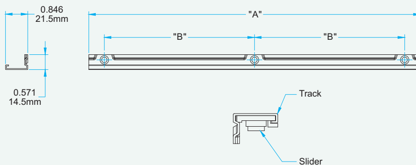
Dual Arm Operator Track 3 Holes
