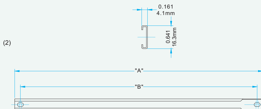
Single Arm Operator Track 2 Holes
