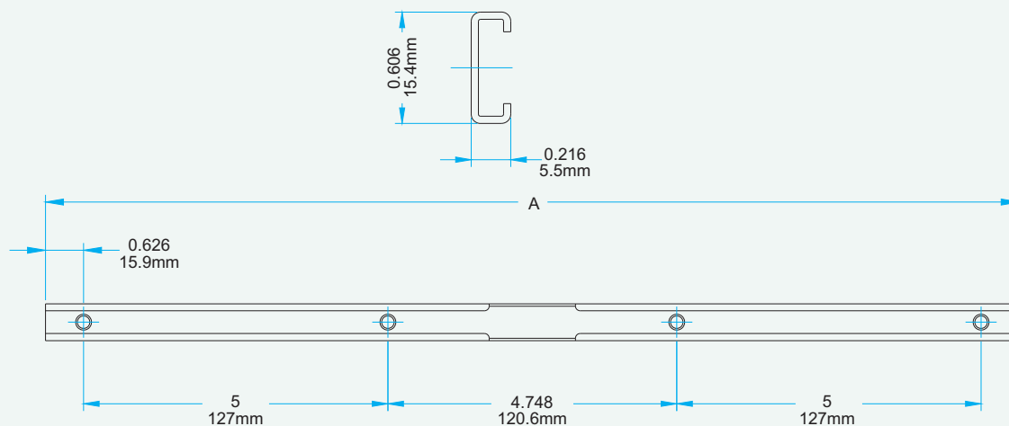
Arming Operator Track 4 Holes
