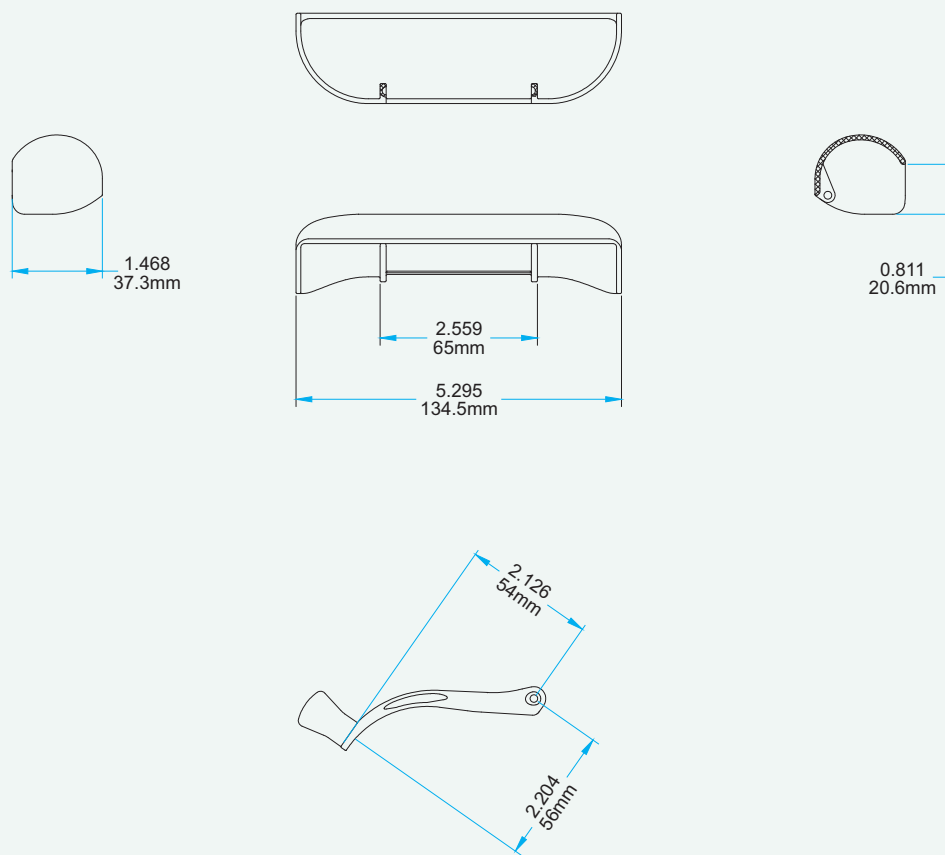
Eclipse Handle / Cover
