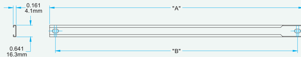
Track
