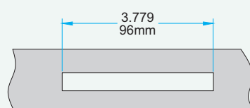
Profile Cut Out (PVC Profile)
