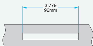
Profile Cut Out (PVC Profile)
