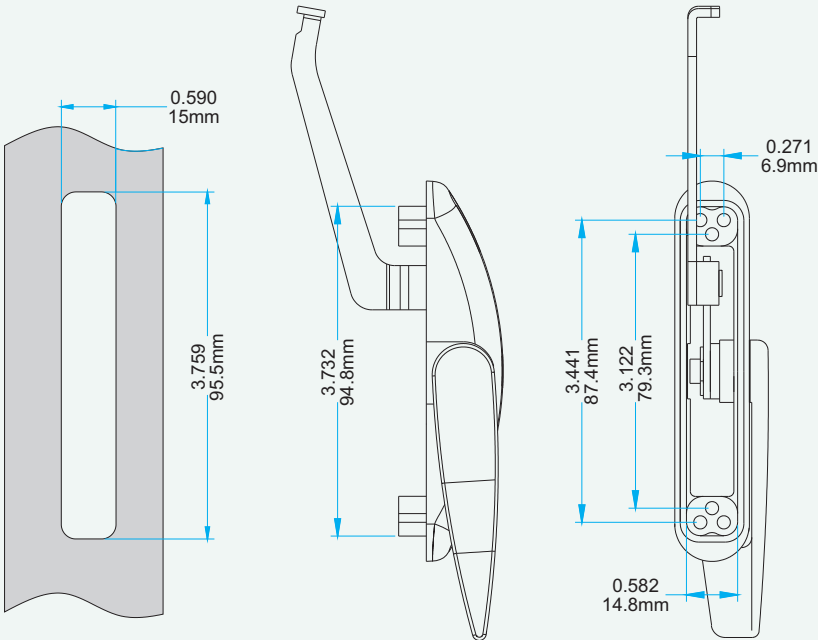
Frame Cut Out
