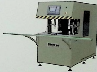
LDJZ1-CNC-6000 塑料门窗数控双区螺钉紧固机 CNC Double Zone Screw Tightening Machine for PVC Doors and Windows
