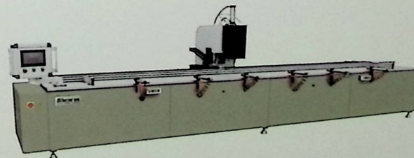
LDJZ1-CNC-6000 塑料门窗数控双区螺钉紧固机 CNC Double Zone Screw Tightening Machine for PVC Doors and Windows
