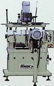
SCX03-3X60 塑料型材自动水槽铣床 PVC Profile Auto Water-slot Milling Machine
