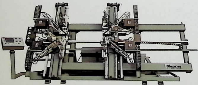
HJ02-4500.4/4A 塑料门窗四点焊接机 PVC Win-door 4-head Welding Machine
