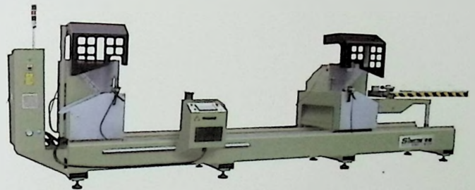
LJZ2F-CNC-550×4200 铝型材数控 45°专用双头精密切割锯床 LJZ2F-CNS-550×4200 铝型材数显 45°专用双头精密切割锯床 CNC 45° Special Double-head Precision Cutting Saw Machine for Aluminum Profile
