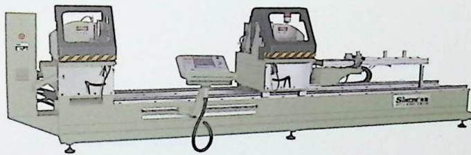
LJZ2B-CNS-500×4200 铝型材双头数显精密切割锯床 Double-head precision cutting saw CNS for aluminum profiles LJZ2B-500×4200 铝型材双头精密切割锯床
