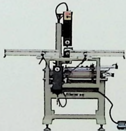
SQJ05-120 塑料门窗 V 形角缝清理机 PVC Win-door V-corner Cleaning Machine
