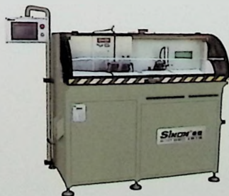
LJJ02-CNC-500 铝门窗数控角码切割锯 Corner Connector Automatic Cutting Saw
