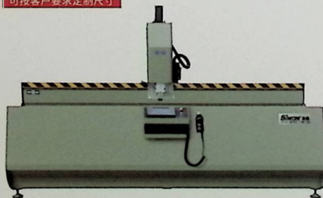
GCGZB-CNC-2500 铝型材数控钻铣加工中心 CNC Drilling and Milling Centers for Aluminum Profiles
