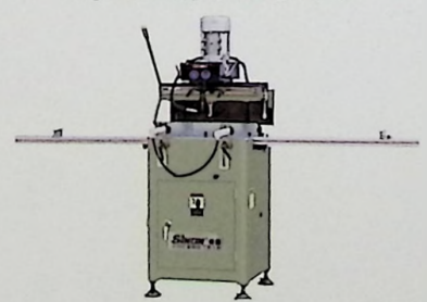
LSXZ1B-125 铝塑型材单轴仿形铣床 Single Head Copying Routing Machine
