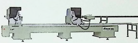
SJT03-420 塑料型材双头切割锯 PVC Win-door Double-head Cutting Saw
