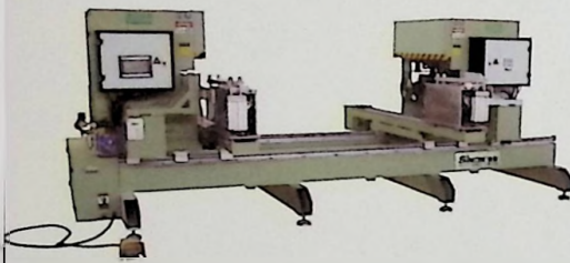
LJKJ-500 铝幕墙接口切割锯床 Aluminum Curtain Wall Notching Saw
