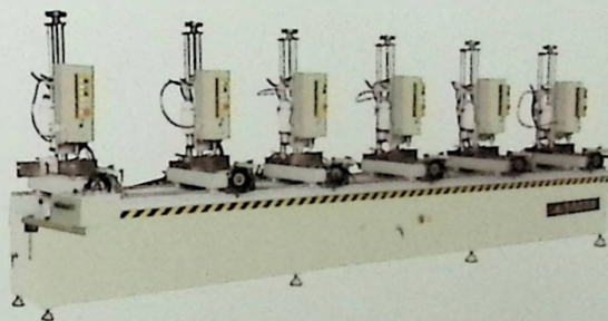
LC-30 铝型材气动冲床 Pneumatic punching machine for aluminum profile
