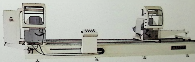
ZXJM-500 铝型材（数显）精密切割锯 Aluminum profile (digital display) precision cutting saw
