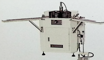
LXDZ-250×5 铝型材超效走刀式自动端面铣床 (五刀) Aluminum profile super-efficient cutter automatic end milling machine (five knives)
