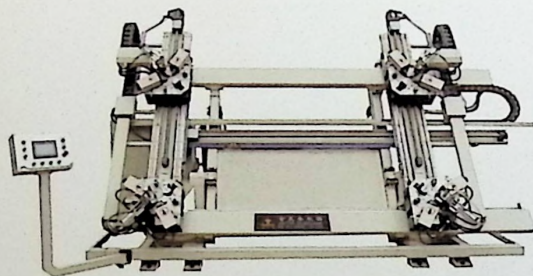
LZJ-120 铝门窗全气动组角机 Aluminum doors and Windows all pneumatic Angle machine
