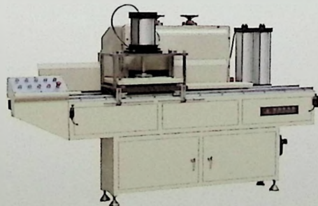
LXD-250×5 铝型材超效自动端面铣床 Aluminum profile super-efficient automatic end milling machine
