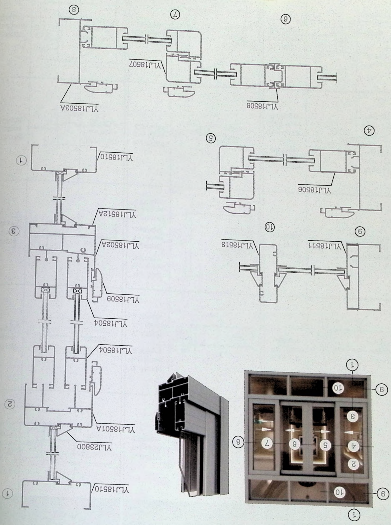
85系列推拉窗(单玻)结构图(新90系列) Structure Diagram of Series 85 Sliding Window(Single)(new 90 series)
