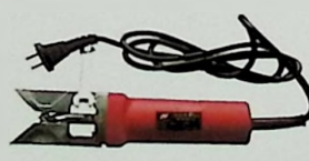
电动塑钢门窗外角清角机 UPVC Window Door External Corner Cleaning Hand Tool
